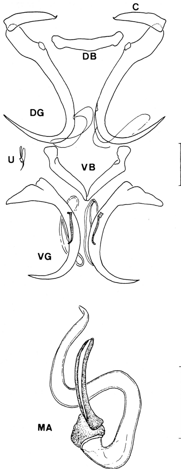
Fig. 2. - Thaparocleidus serpens n. sp. C = cuneus; DB = dorsal transverse bar; DG = dorsal gripus; MA = male apparatus; VB = ventral transverse bar; VG = ventral gripus, U = uncinulus. Bar = 30 µm.
