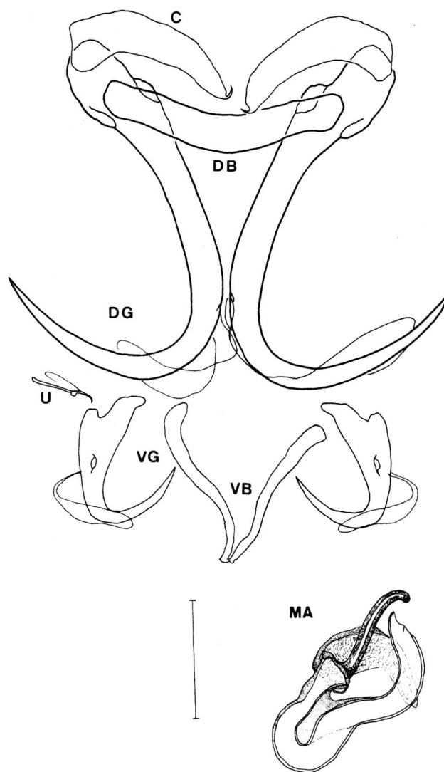
Fig. 3. – Thaparocleidus ocrea n. sp. C = cuneus; DB = dorsal transverse bar; DG = dorsal gripus; MA = male apparatus; VB = ventral transverse bar; VG = ventral gripus; U = uncinulus. Bar = 30 \mu m.
